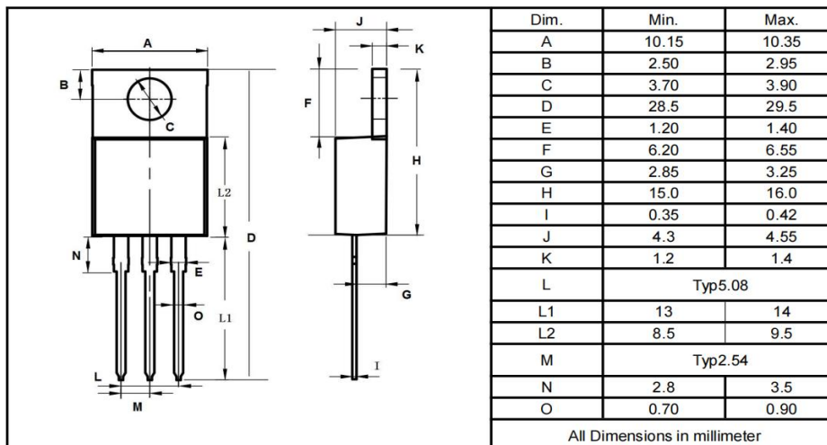
TO-220AB
